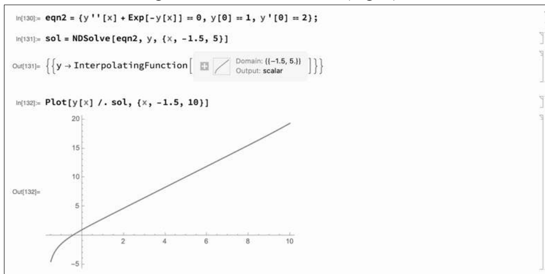
Fig. 3. A numeric solution of a second-order differential equation
